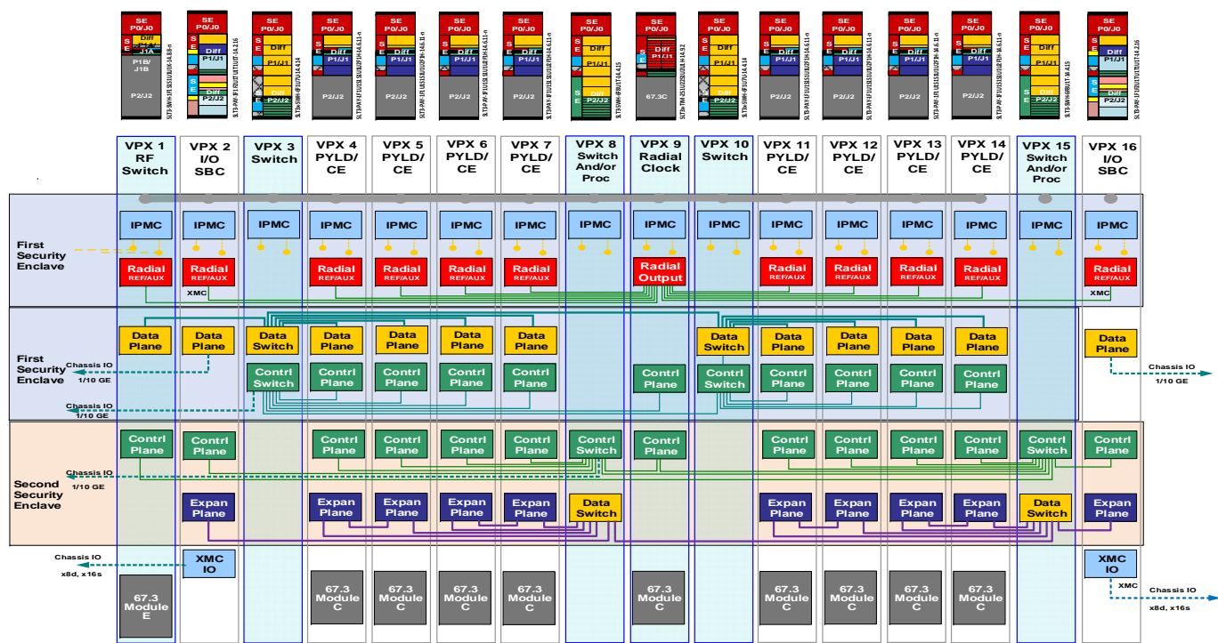
16 Slot Backplane
